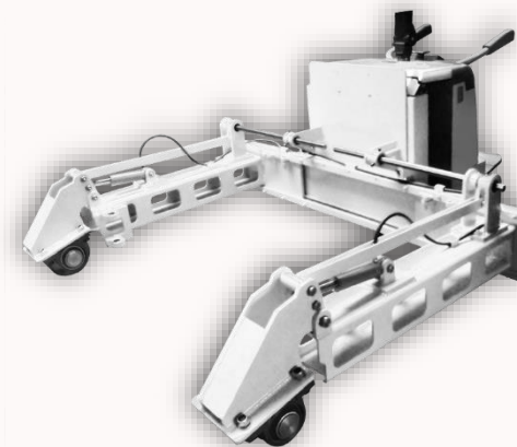
TRANSPORT TROLLEYS
