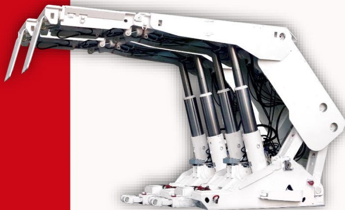
MECHANISED SUPPORTS
